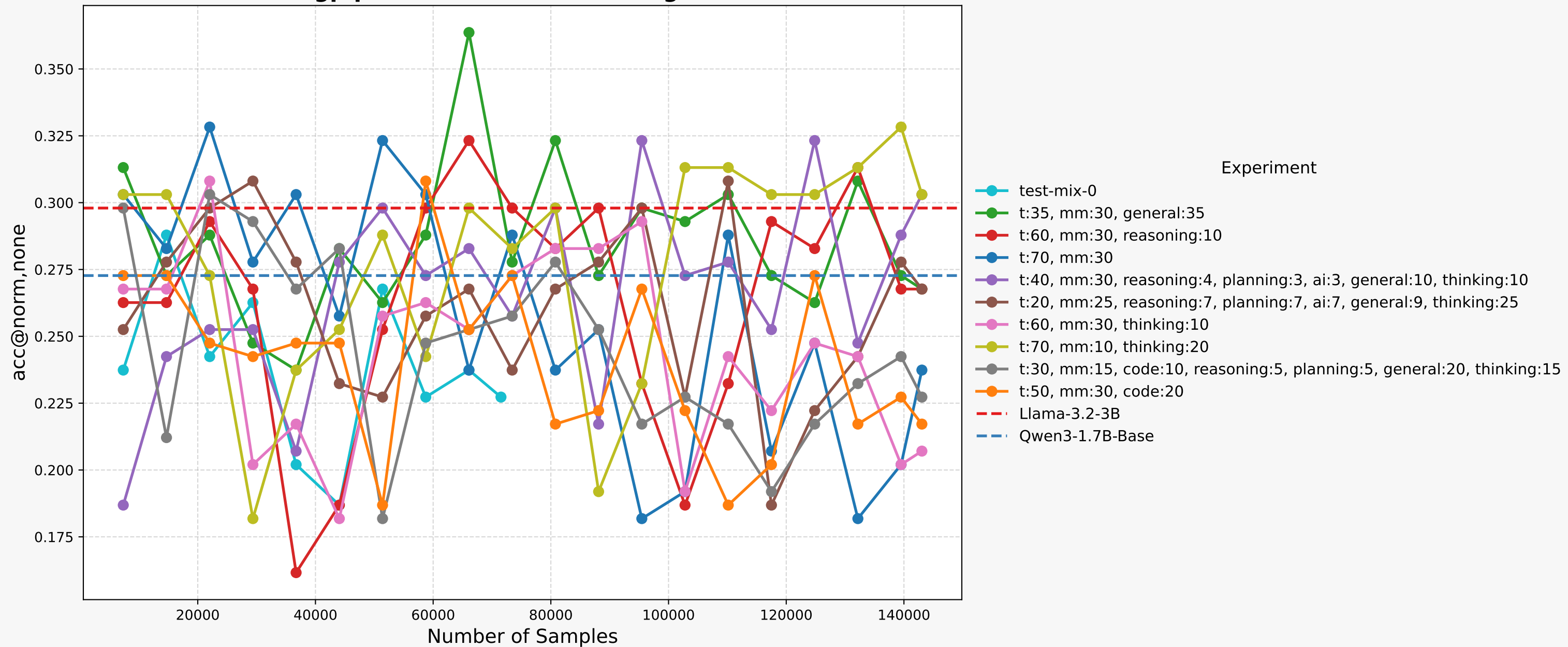
gpqa Tokenmix Ablation Progress
