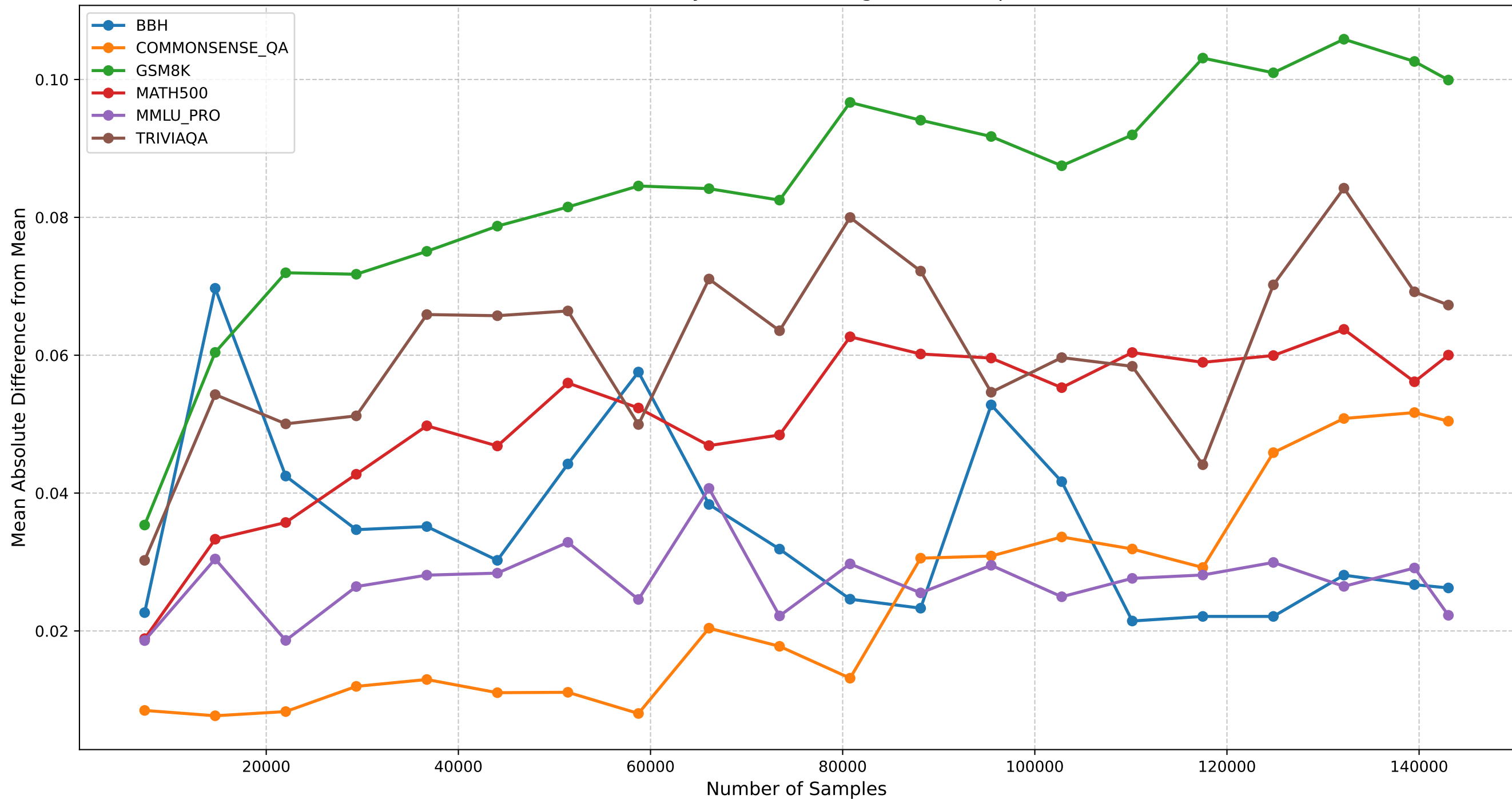
Mean Absolute Difference Across Checkpoints for Each Benchmark (Normalized by Qwen3, Averaged Across Splits)
