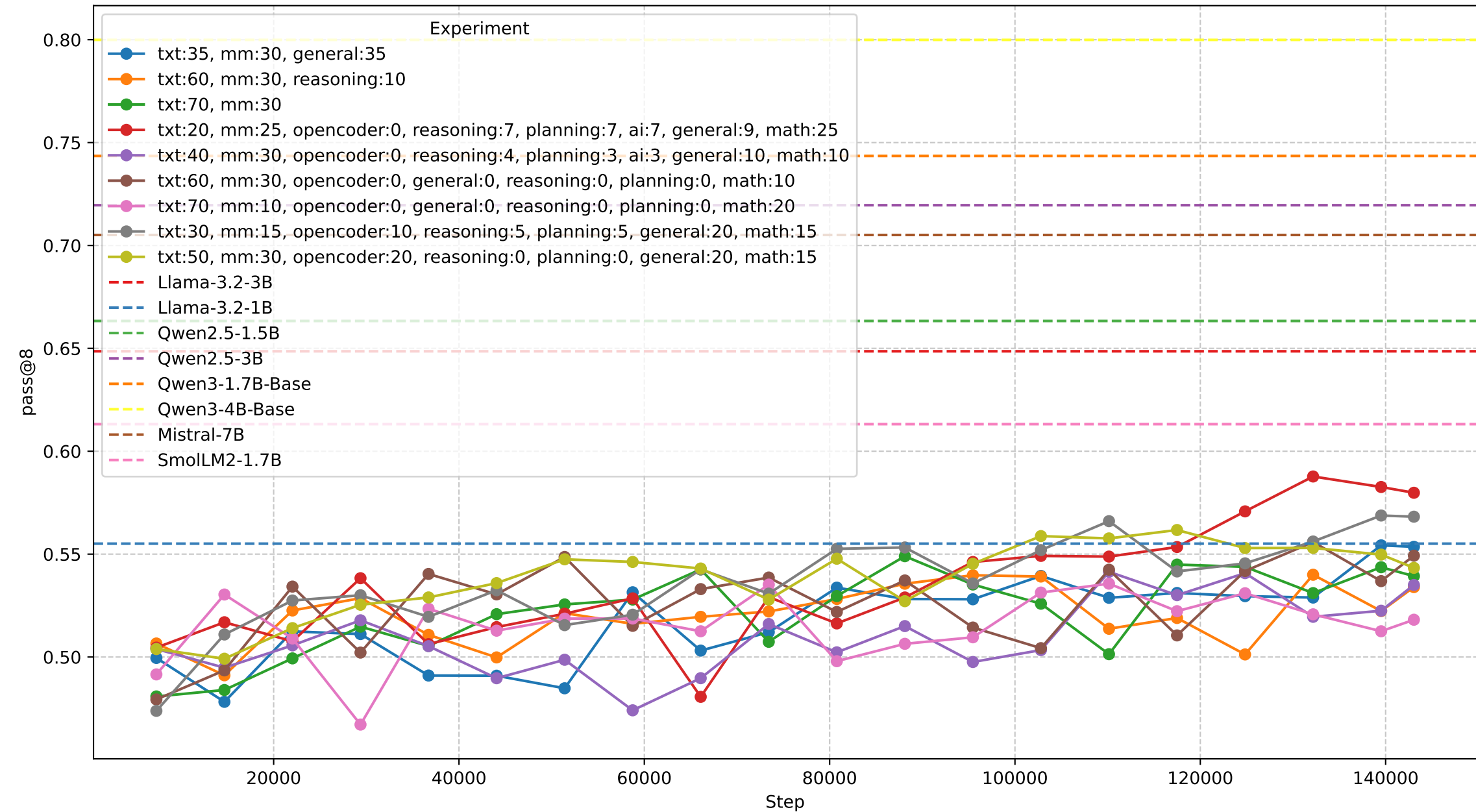
pass@8 vs Step
