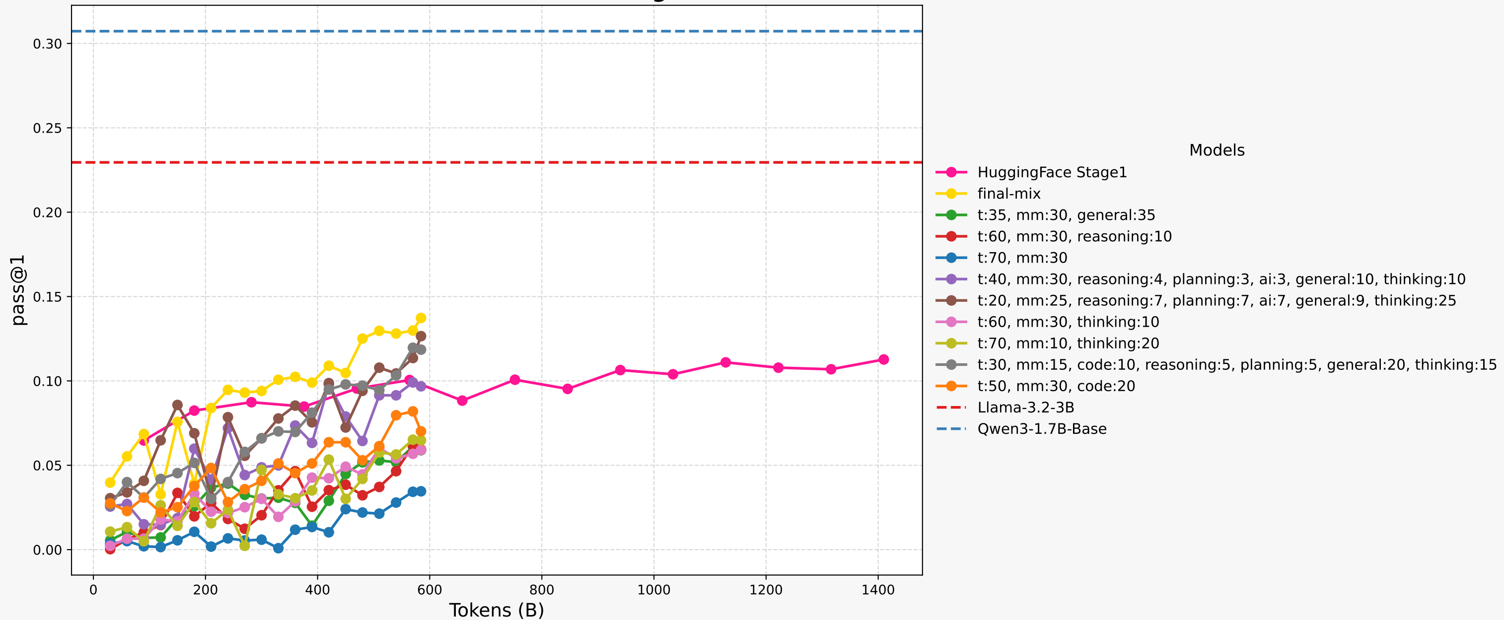
humaneval Performance vs Training Tokens
