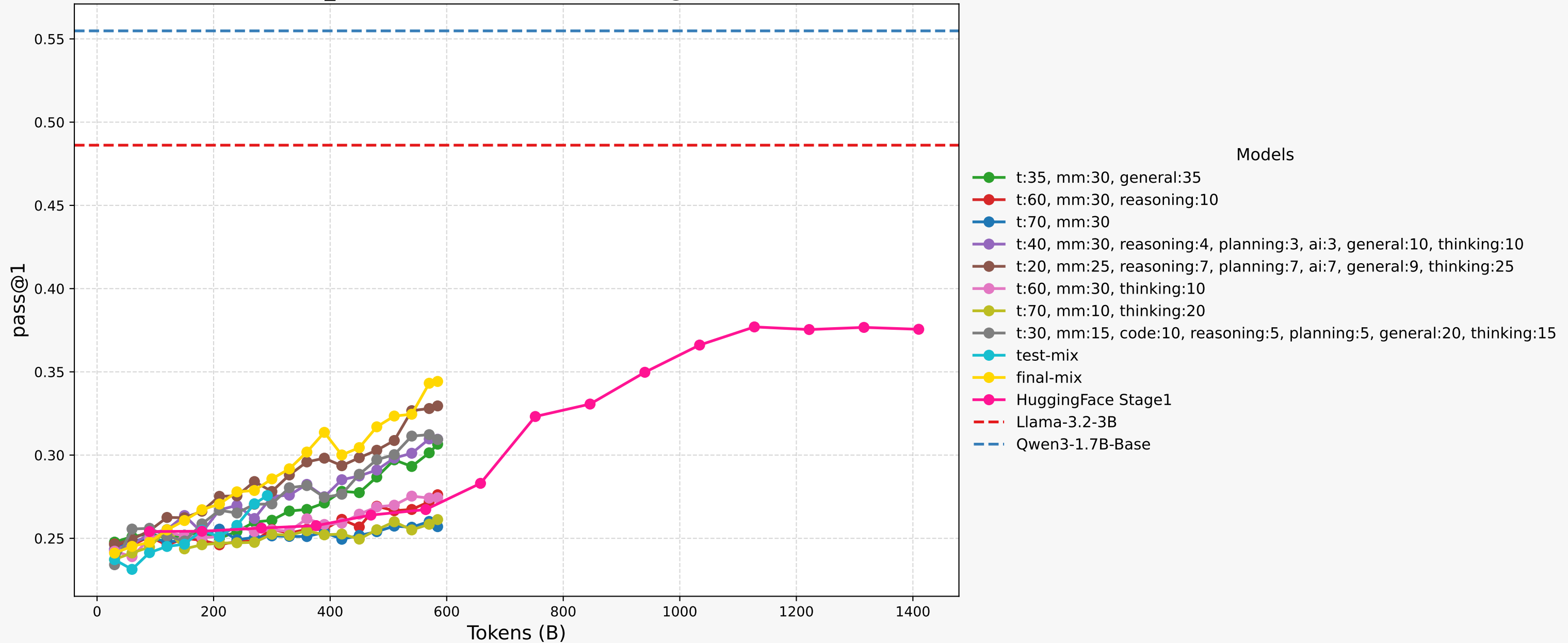
mmlu_std Performance vs Training Tokens
