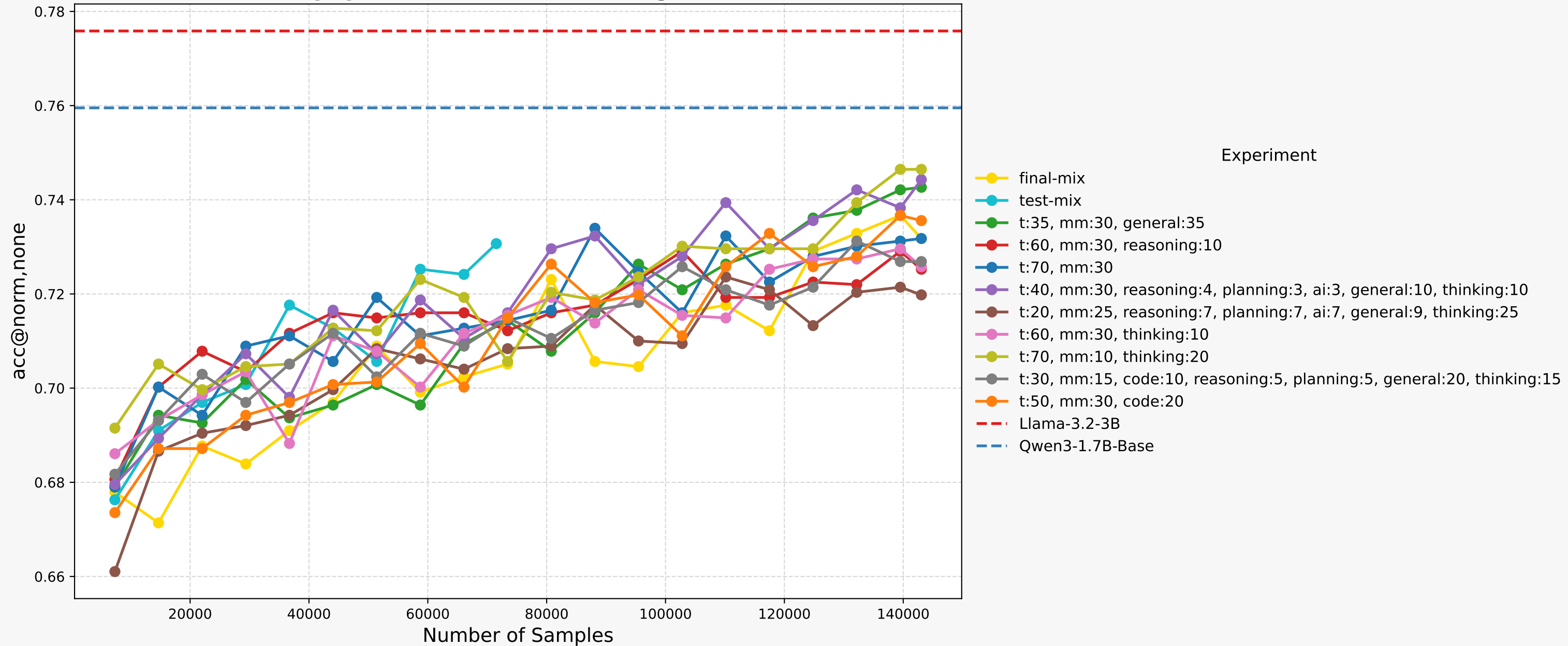
piqa Tokenmix Ablation Progress
