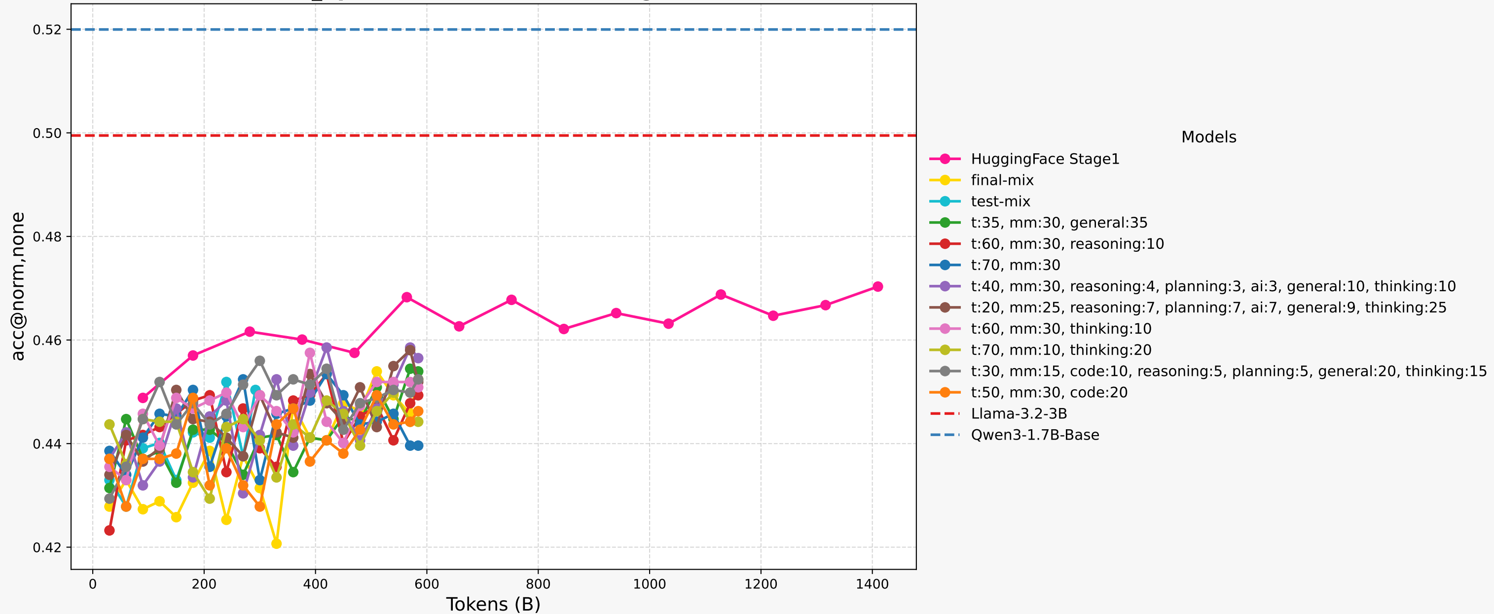
social_iqa Performance vs Training Tokens
