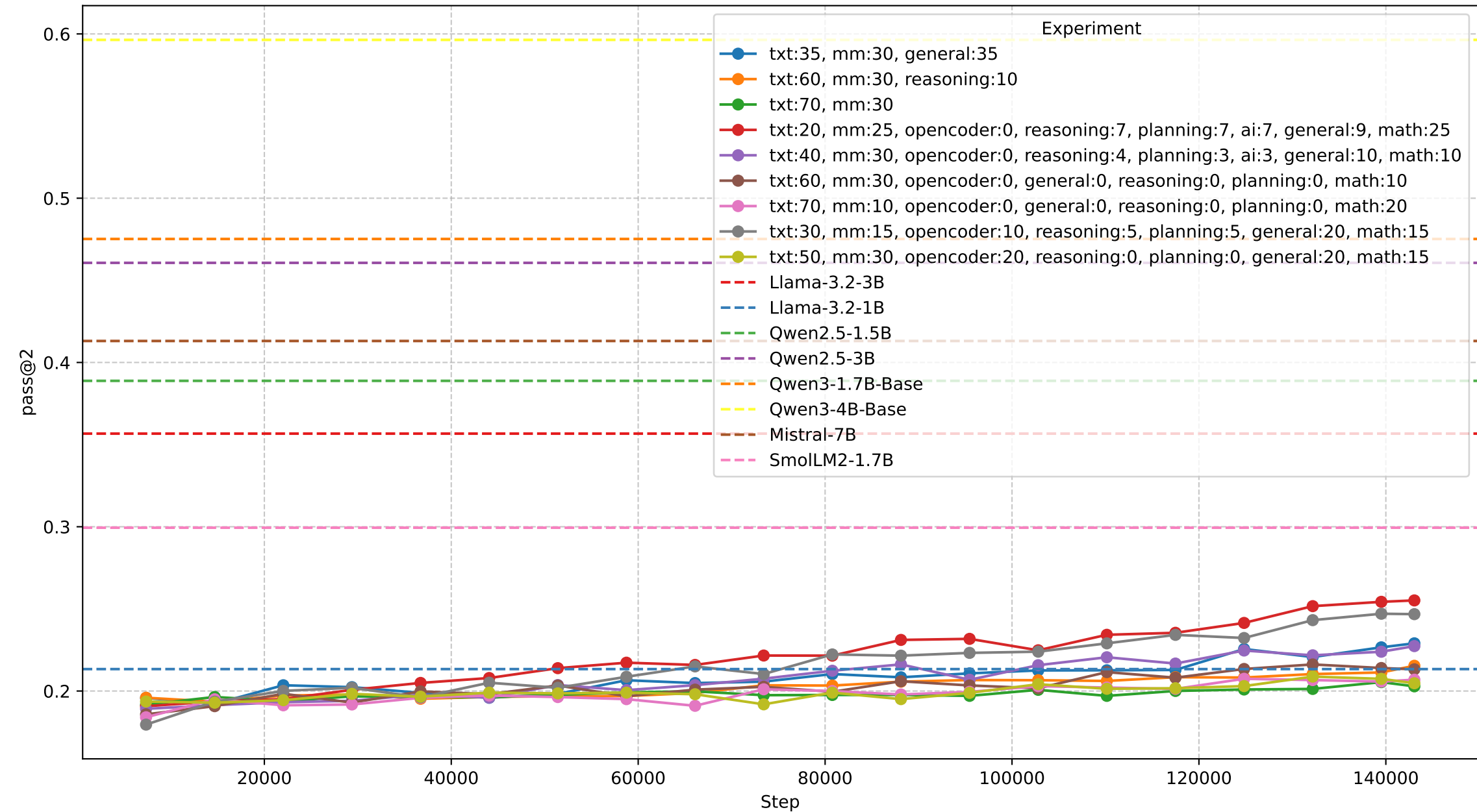
pass@2 vs Step
