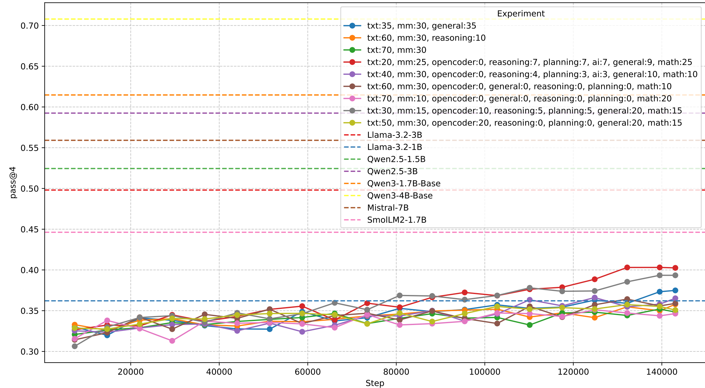
pass@4 vs Step
