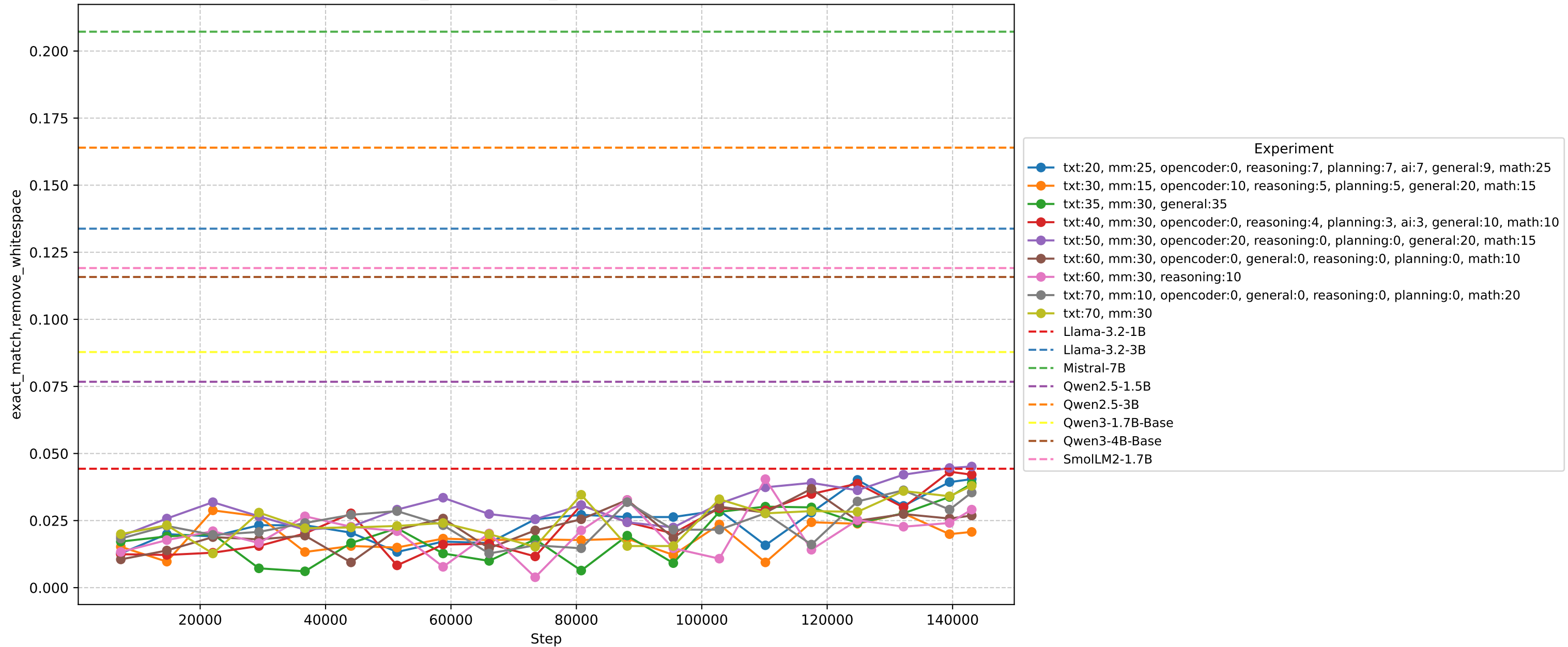
exact_match,remove_whitespace vs Step
