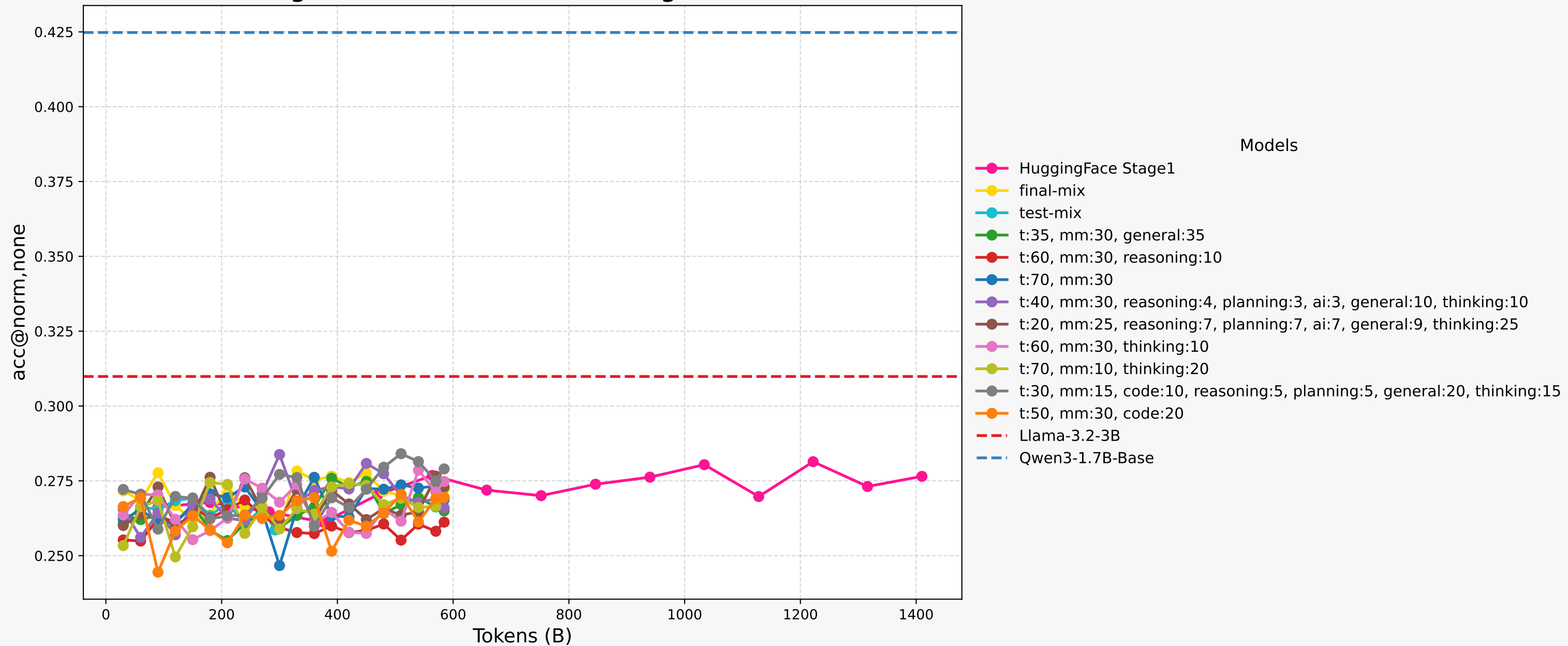
agieval Performance vs Training Tokens
