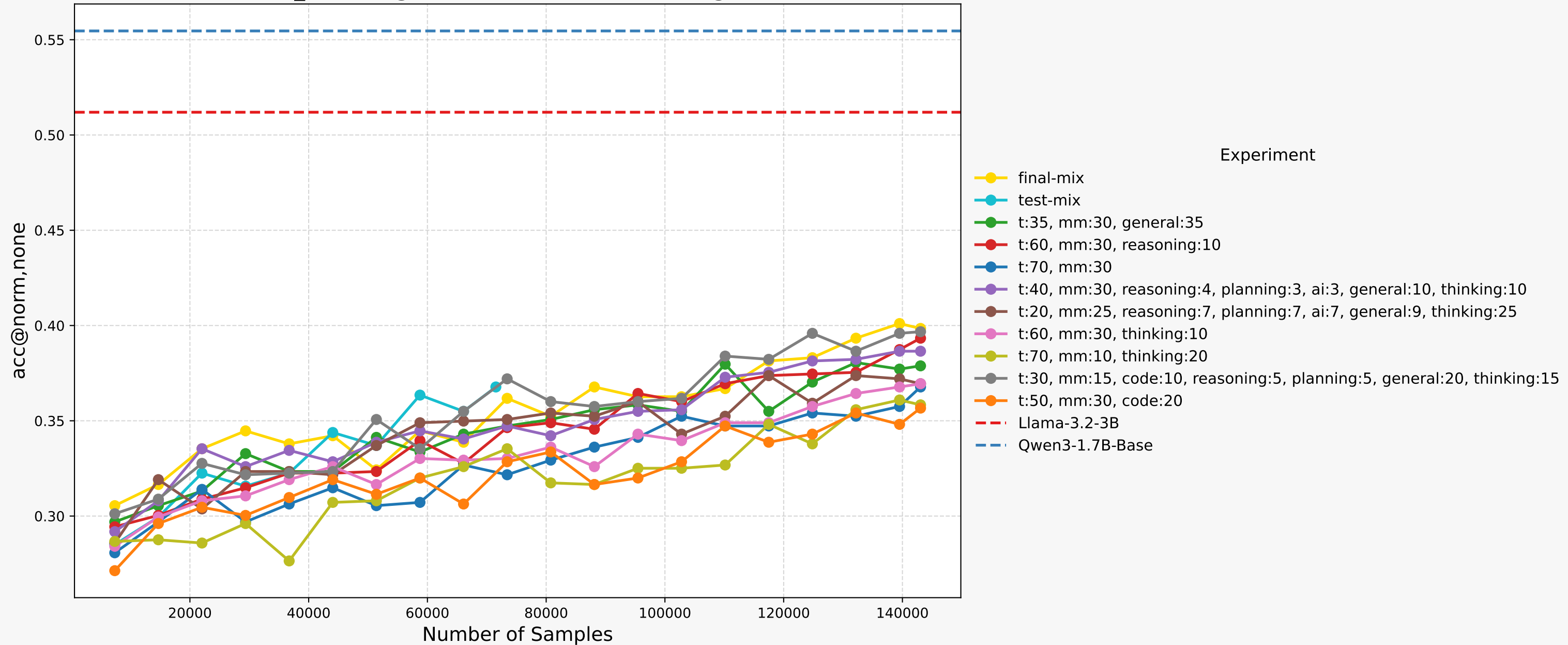
arc_challenge Tokenmix Ablation Progress
