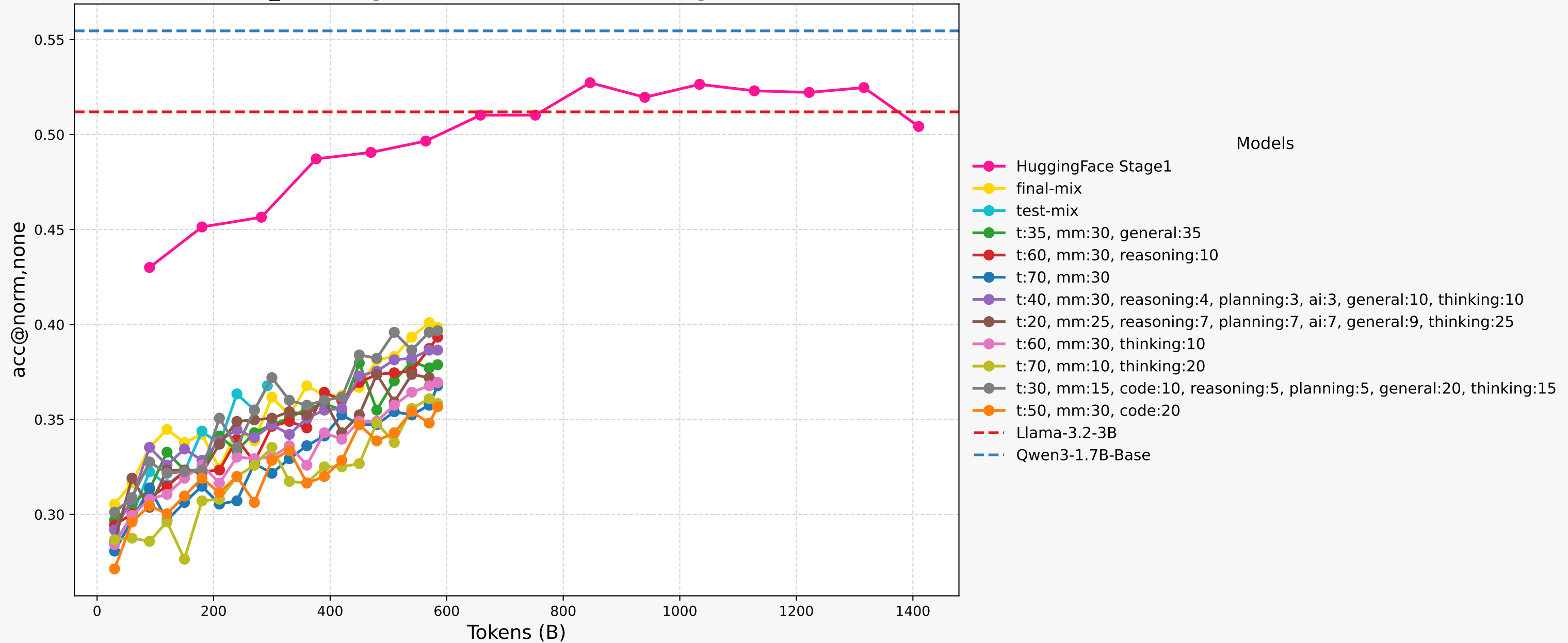
arc_challenge Performance vs Training Tokens
