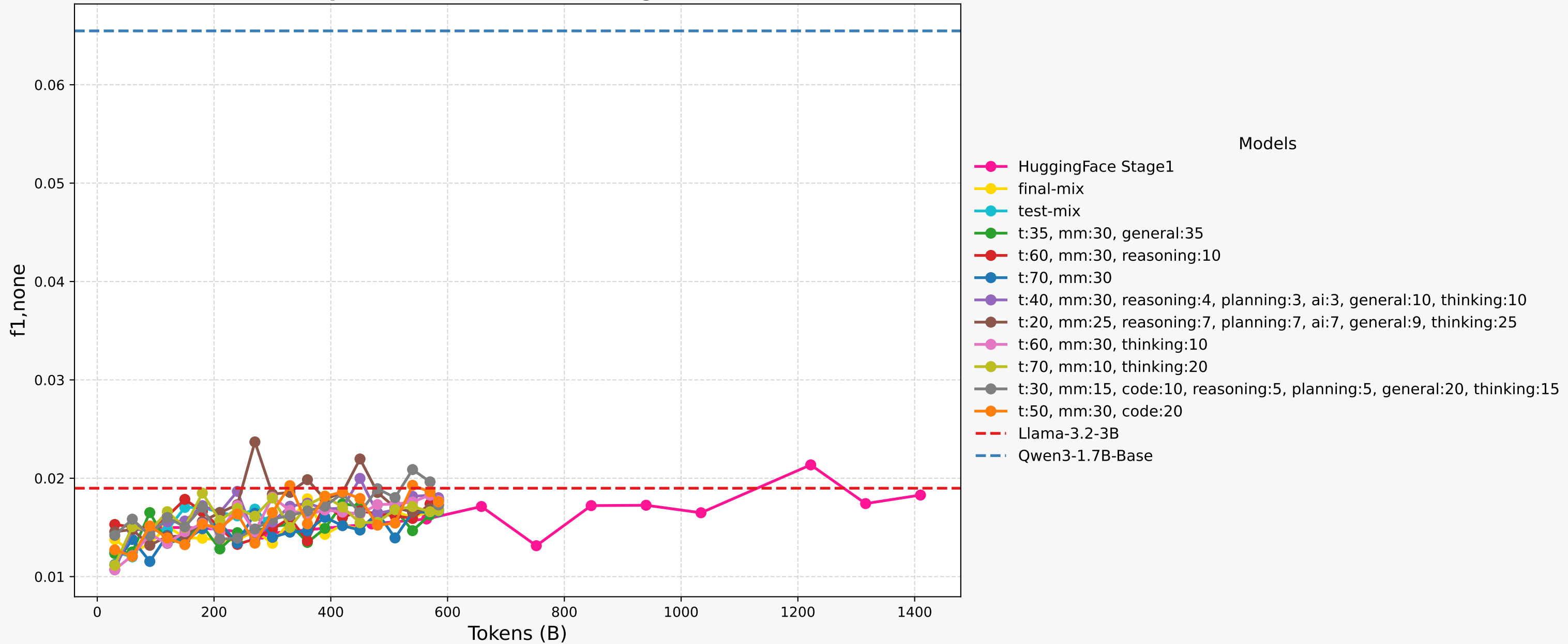
drop Performance vs Training Tokens
