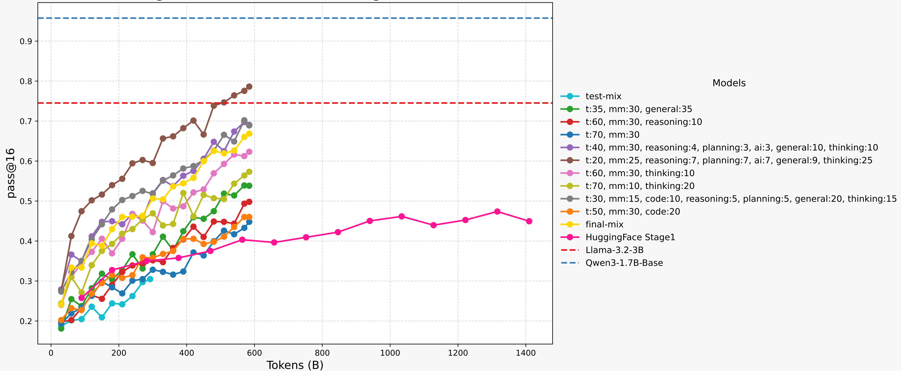
gsm8k Performance vs Training Tokens
