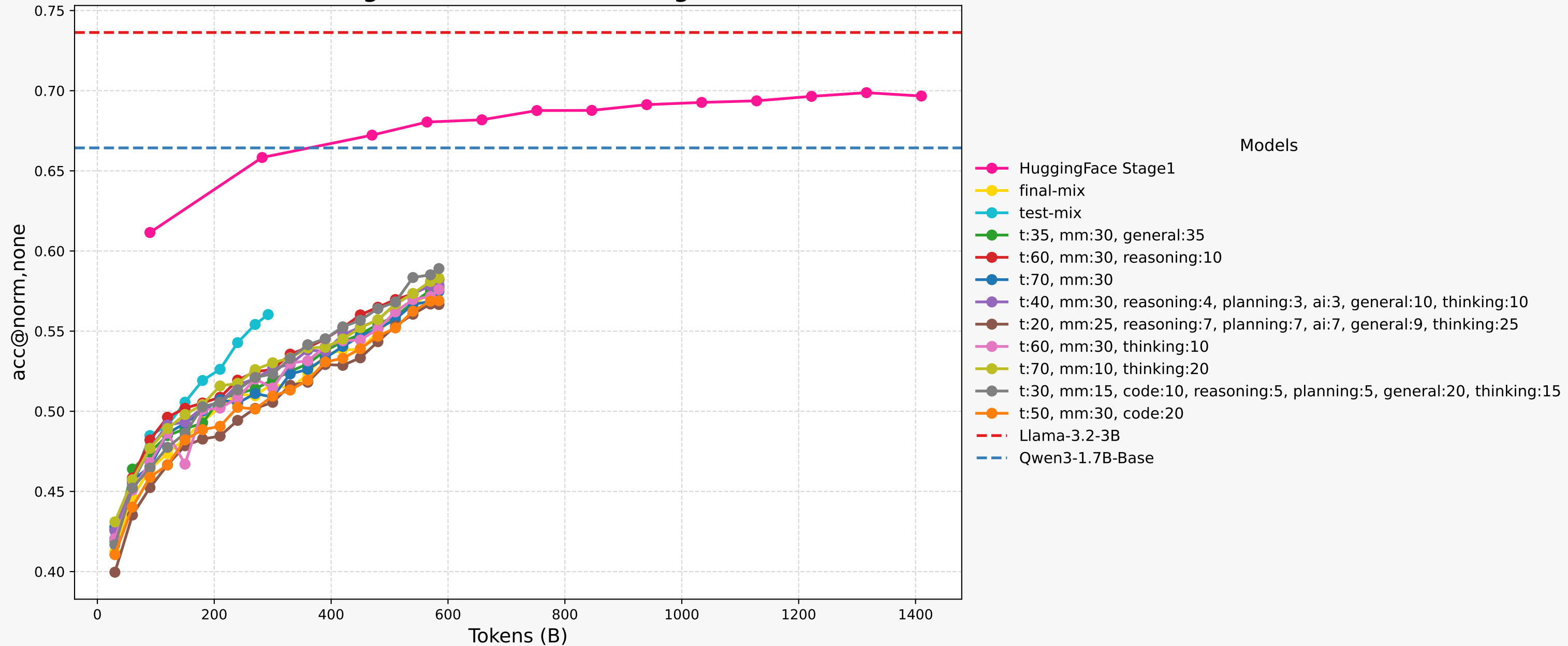
hellaswag Performance vs Training Tokens
