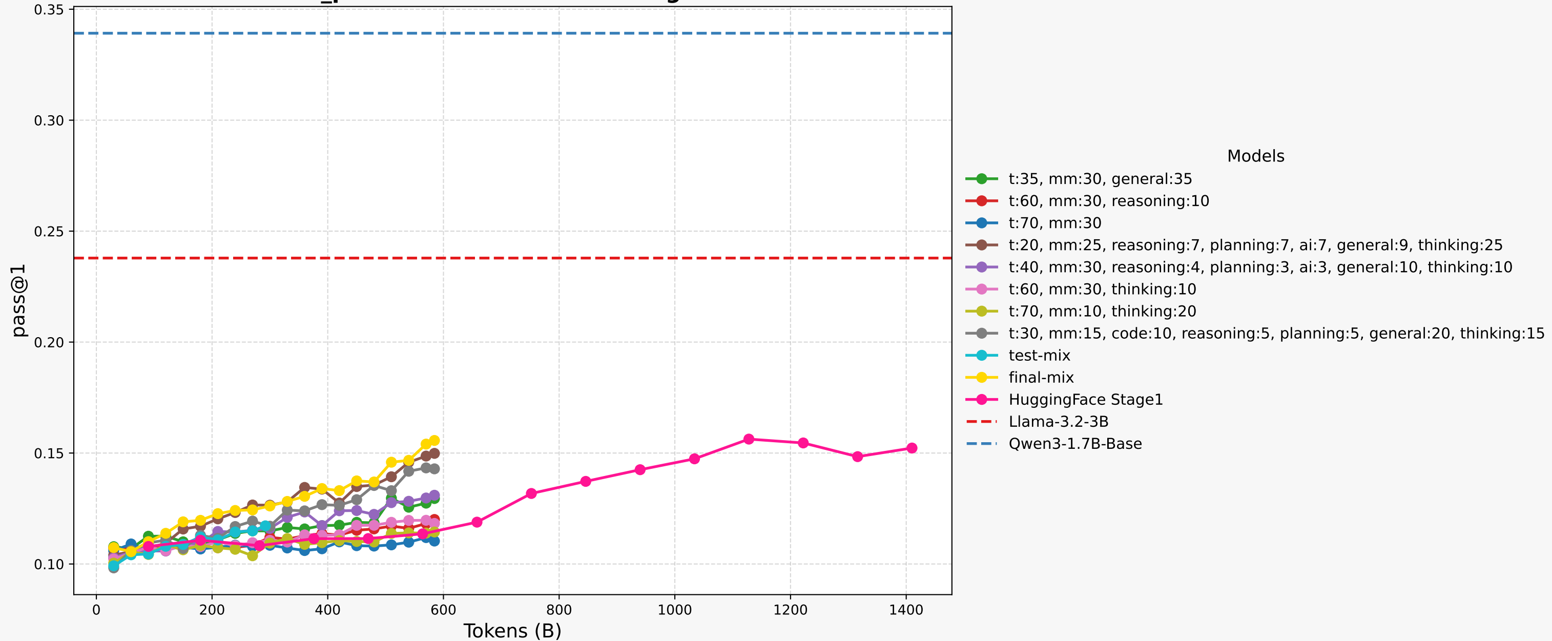
mmlu_pro Performance vs Training Tokens
