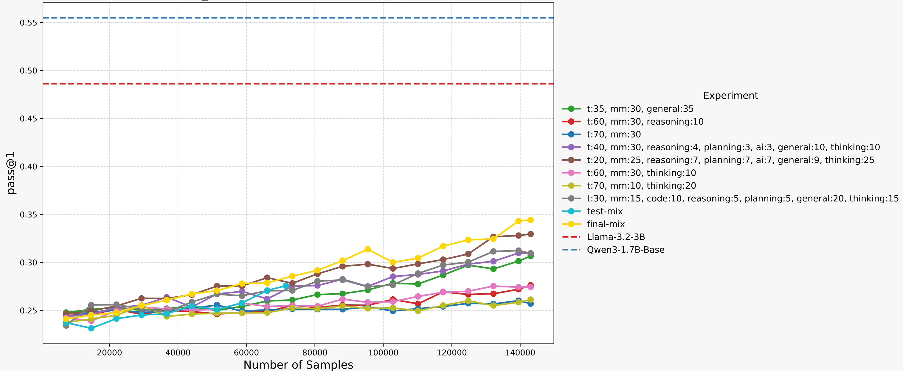
mmlu_std Tokenmix Ablation Progress
