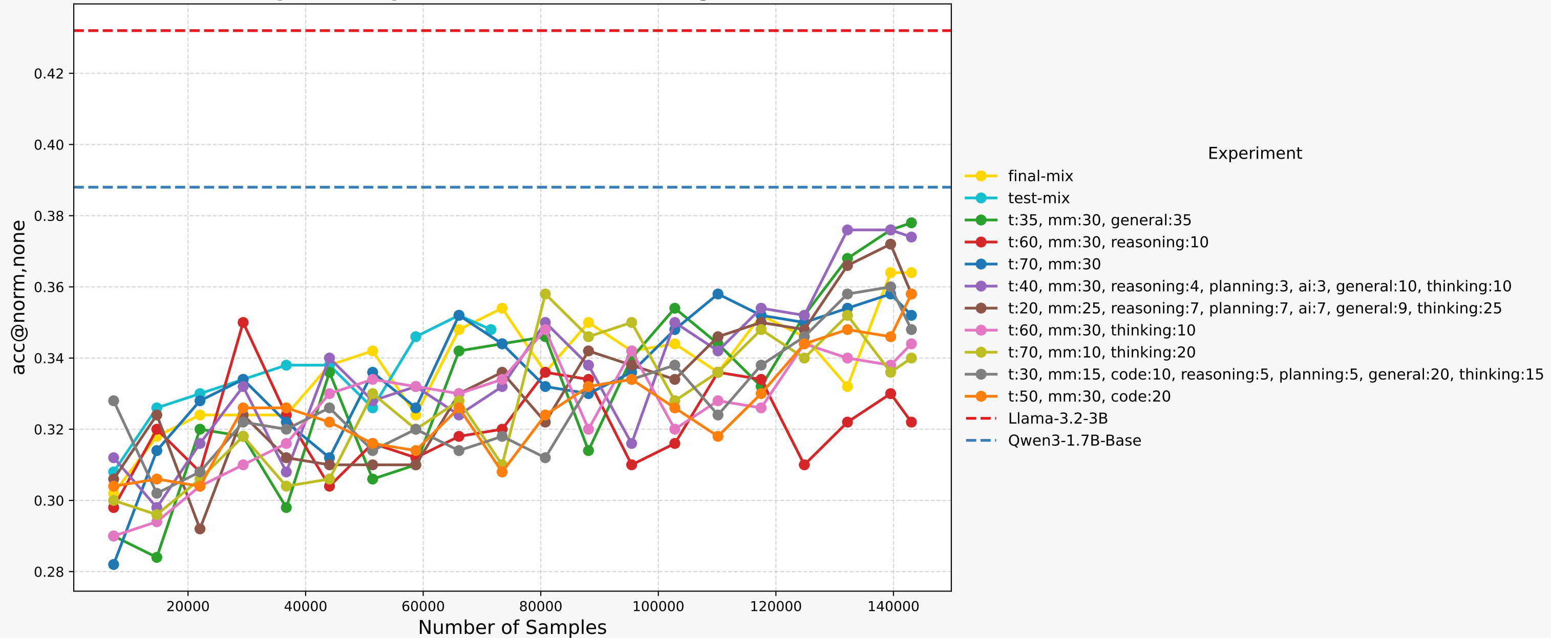
openbookqa Tokenmix Ablation Progress
