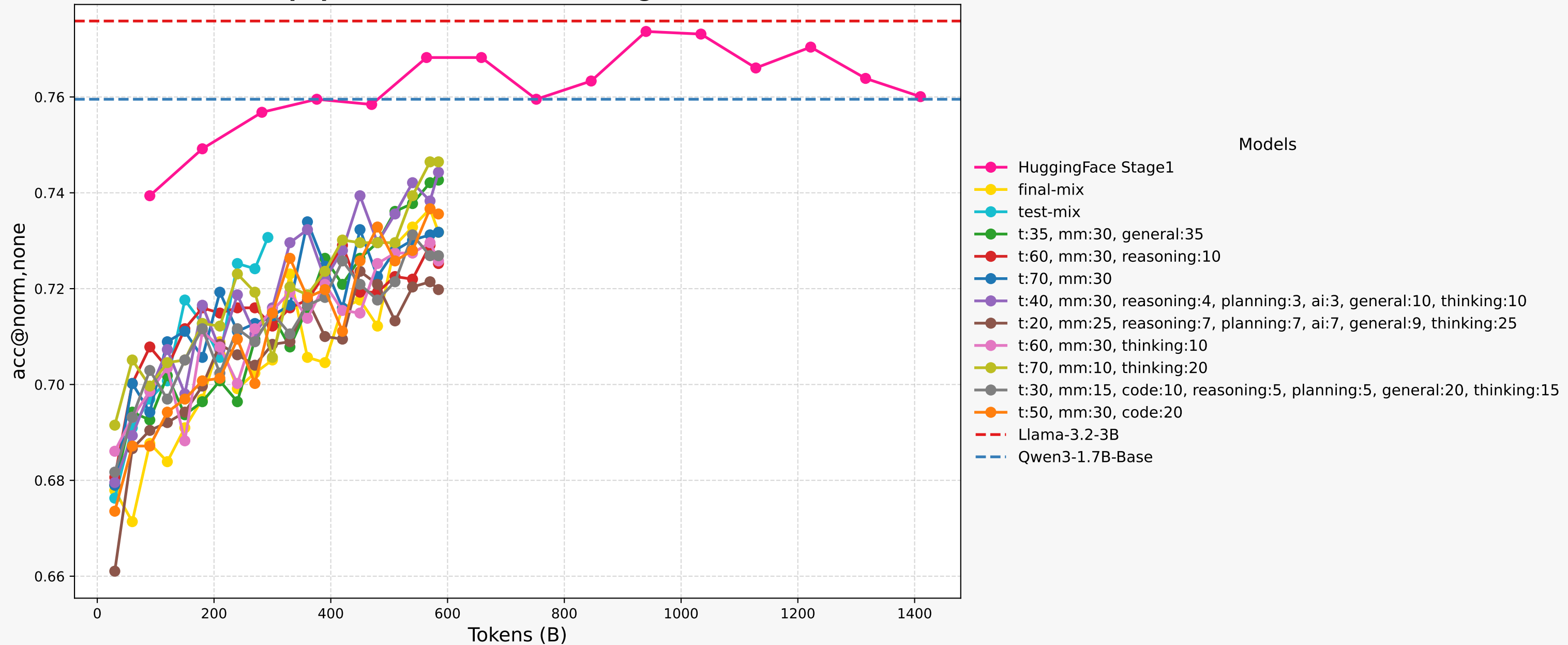
piqa Performance vs Training Tokens
