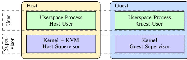
Figure 1. On x86-64 systems with VMs, protection domains include HU, HS, GU, and GS, extending beyond user and supervisor modes.
