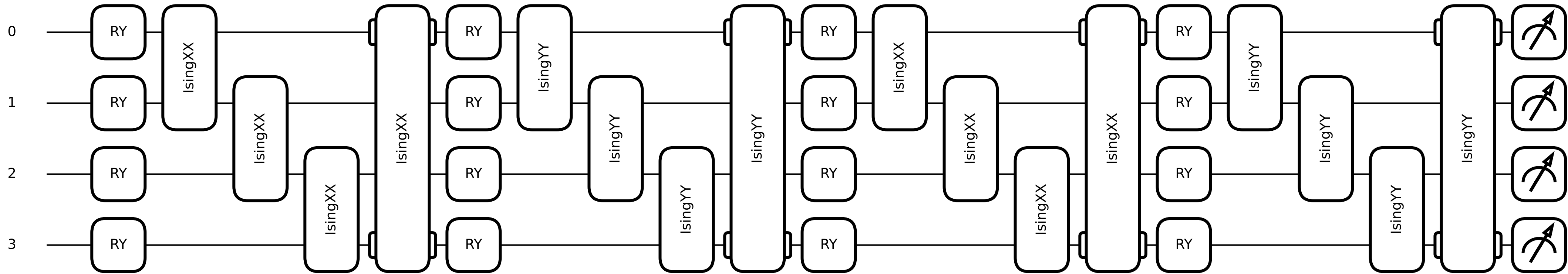
QLCU Circuit (4 Qubits, 2 Layers)
