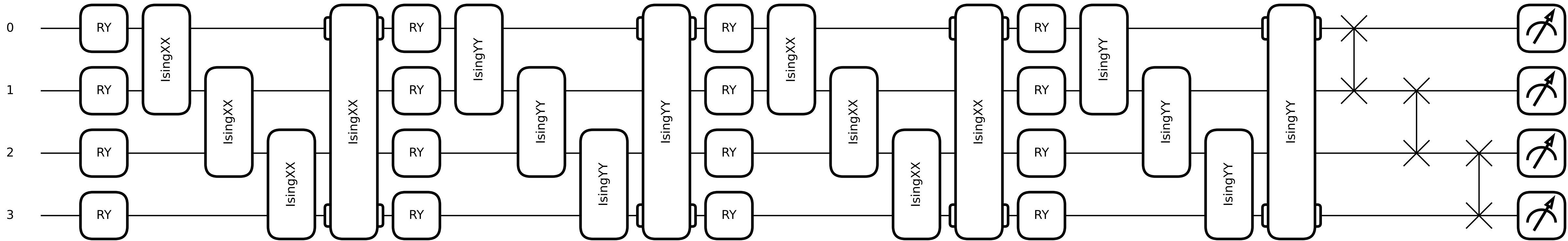
Hydra Branch \psi_1 : Qshift(QLCU|X>)
