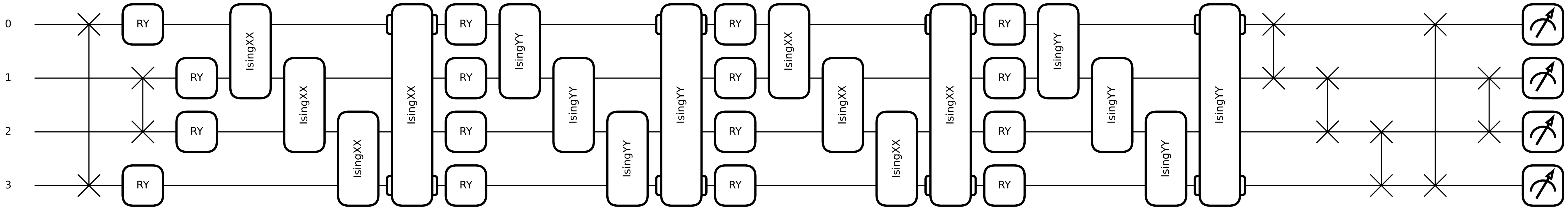
Hydra Branch \psi_2 : Qflip(Qshift(QLCU(Qflip|X))))
