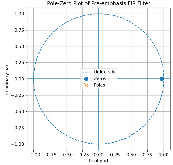
Fig. 5. Pole-zero plot of the pre-emphasis FIR filter.
