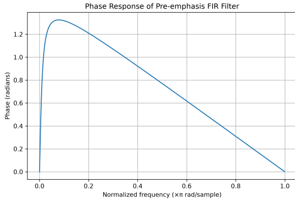
Fig. 7. Phase response of the pre-emphasis FIR filter.
