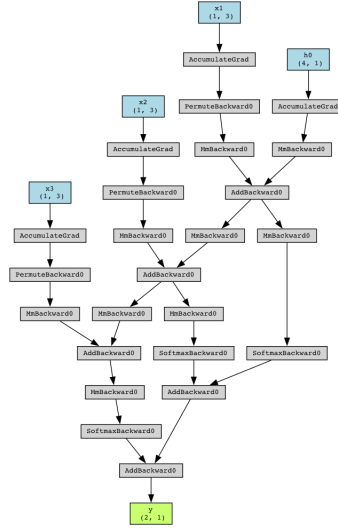
Figure 2: Q2.1 Computation graph.
