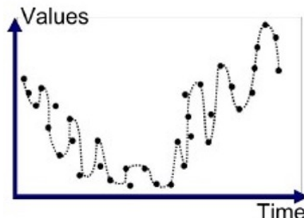
Overfitted
