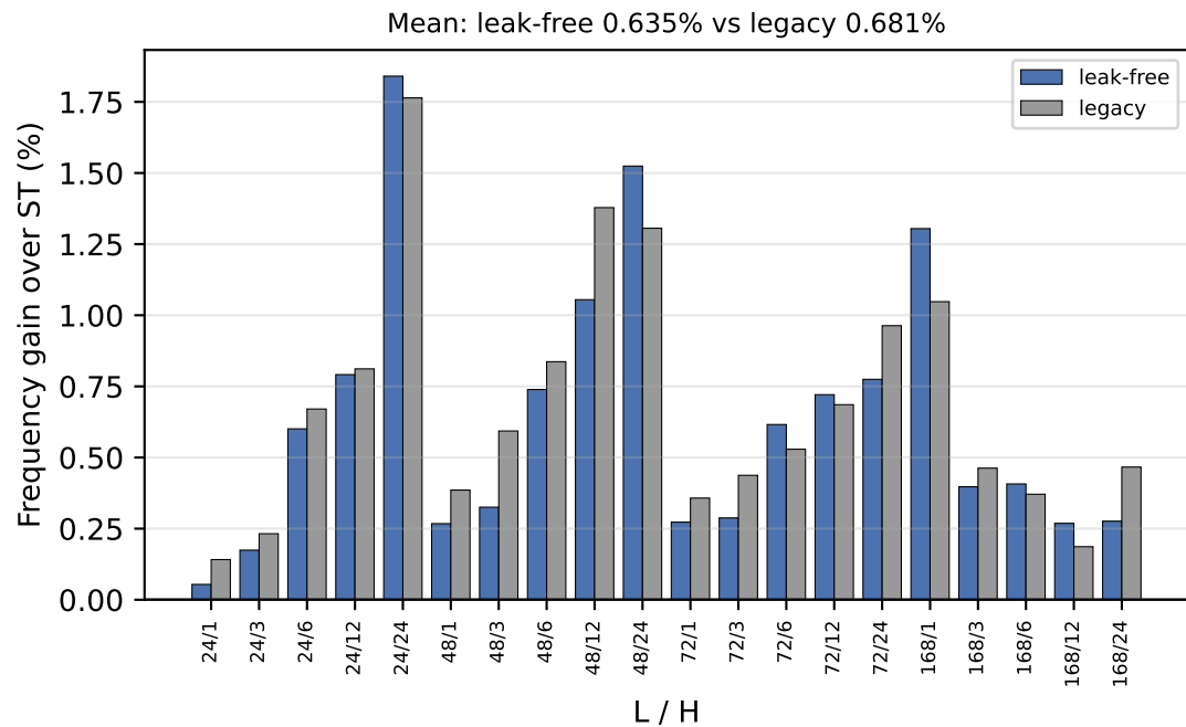
Beijing frequency arms: leak-free vs legacy pipeline (20 configs, 5 seeds)
