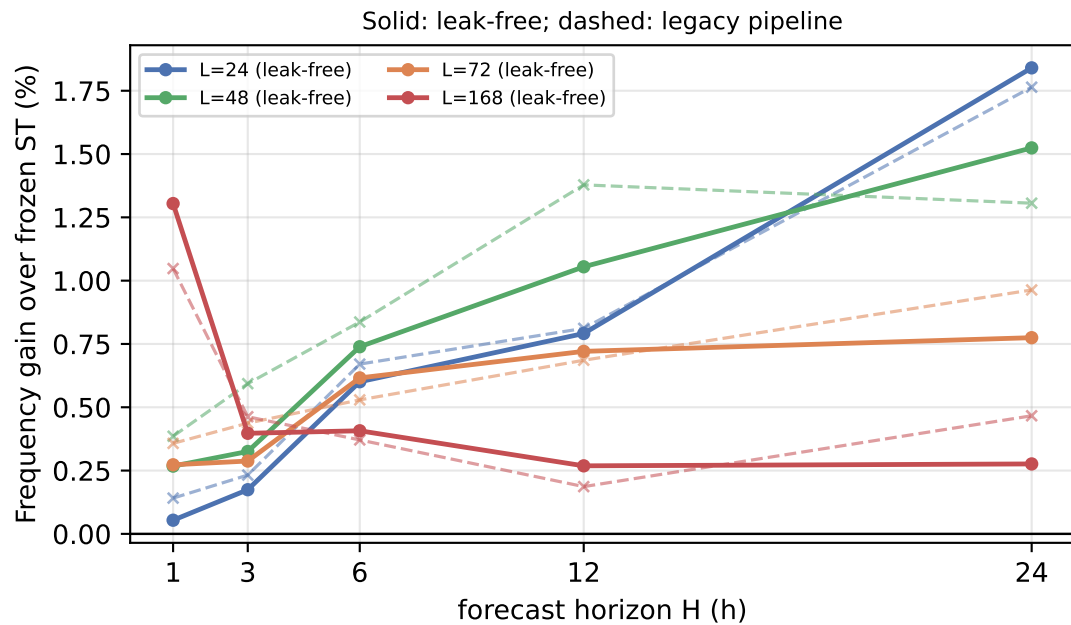
Beijing frequency arms: leak-free vs legacy pipeline (20 configs, 5 seeds)
