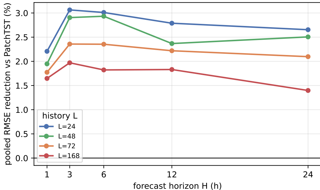
Guangzhou: spatial structure gain vs horizon
