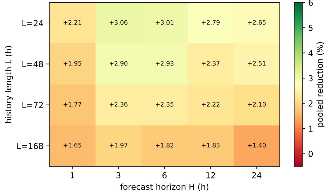
Gain grid (8 stations × 5 seeds, pooled)
