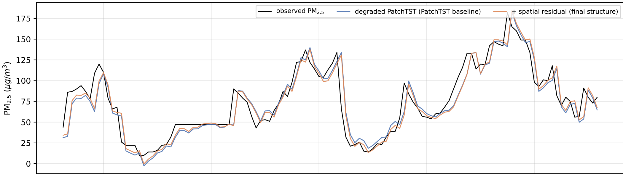
Beijing station 1013, seed 2047, 168 \rightarrow 6, test split; illustrative re-run (RMSE 22.552 vs 22.195, reduction 1.58%)
