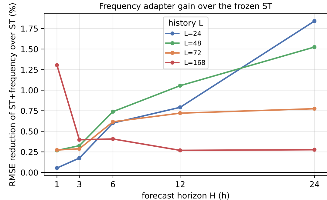
Frequency adapter across history lengths and horizons (5 seeds, test split)
