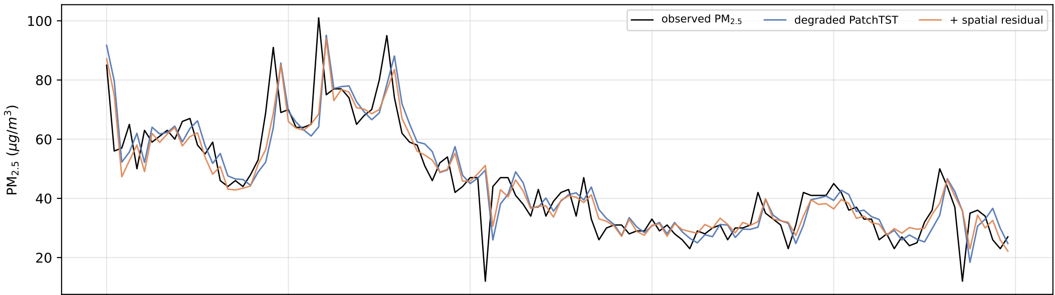
Guangzhou station 9033, seed 7001, 24 → 1; first confirmation block (RMSE 7.522 vs 6.688, reduction 11.08%)
