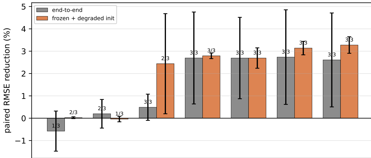
24 → 1 — component ablation (test split, seeds 2024-2026)
