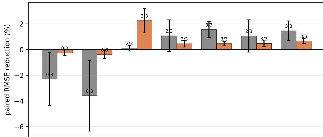
168 → 6 — component ablation (test split, seeds 2024-2026)
