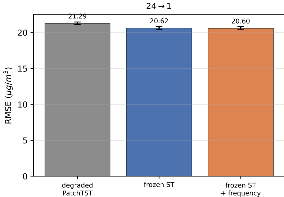
Test-split RMSE: degraded PatchTST, frozen ST, and frozen ST + frequency residual (mean \pm sd over seeds 2047-2051)
