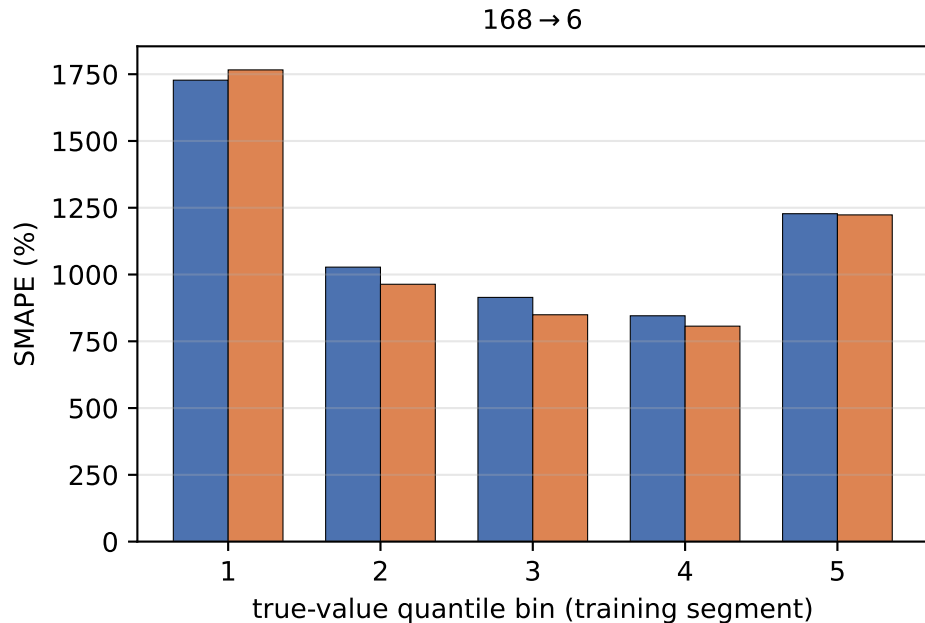
SMAPE by true-value quantile bin (pooled over stations and seeds)
