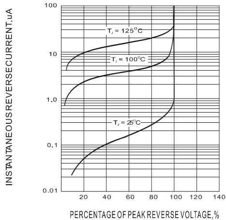
Fig.3-TYPICAL REVERSE CHARACTERISTIC
