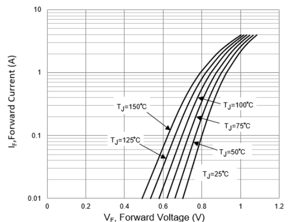
Fig.6 GS1G-AU TYPICAL FORWARD CHARACTERISTICS
