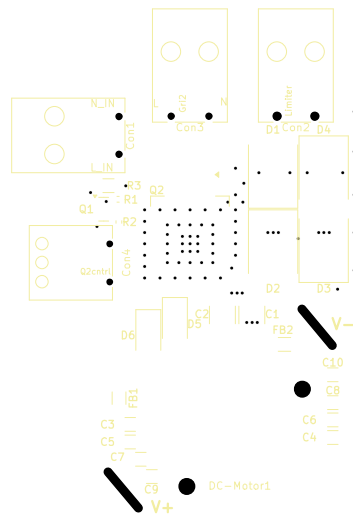
Triac_on_Grinder_v2.1
