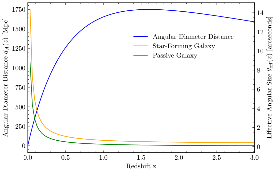
Angular Diameter Distance and Effective Angular Size vs Redshift
