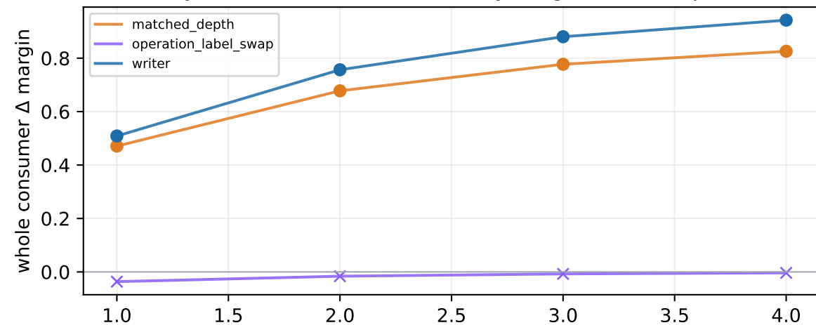
qwen: Qwen/Qwen2.5-1.5B family-local scale; no cross-family magnitude comparison
