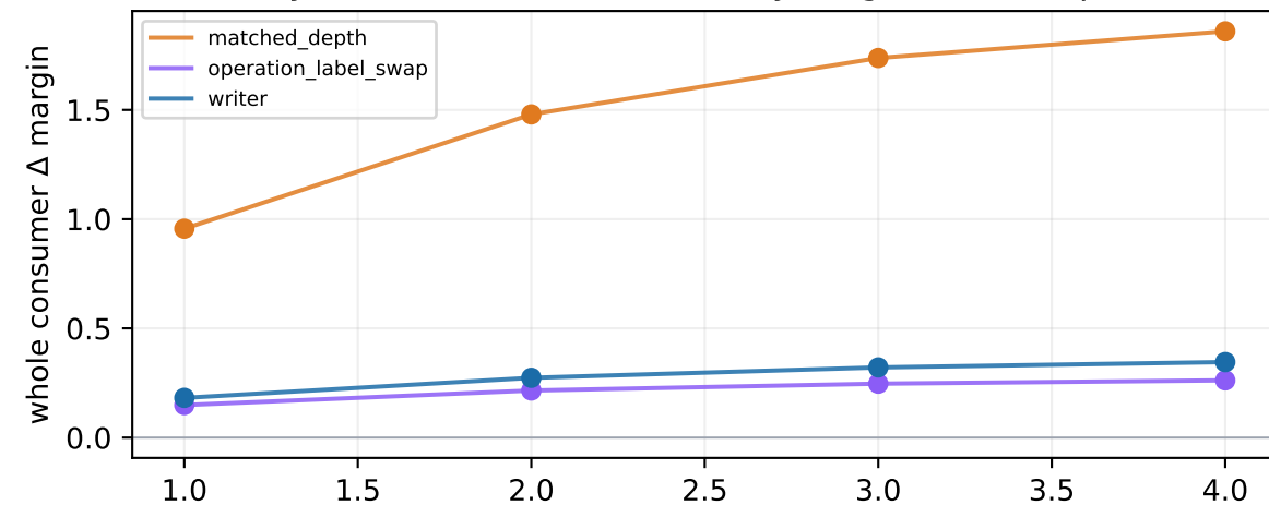
mamba: state-spaces/mamba-130m-hf family-local scale; no cross-family magnitude comparison
