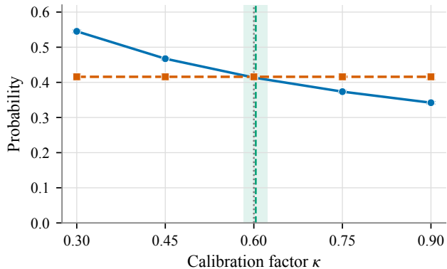
(a) No-new-feasible-entry probability
