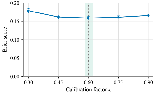
(b) Probability calibration
