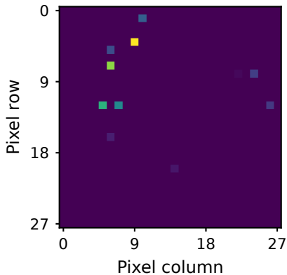
(b) Myopic Q
