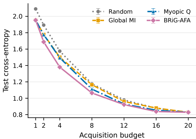
(b) Fashion-MNIST
