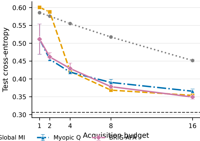
(b) Cross-entropy
