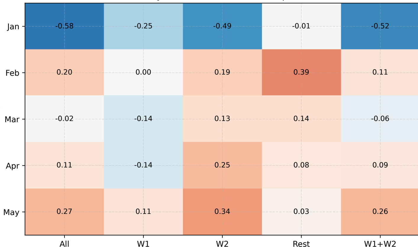
Monthly Z300 ACC vs EP100 components
