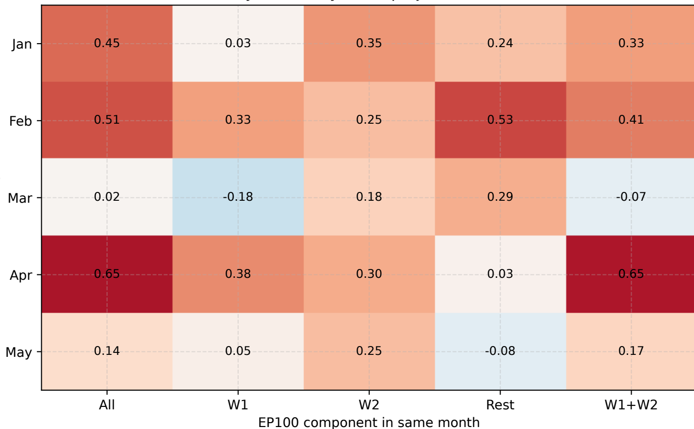
Monthly stationary-wave projection vs EP100
