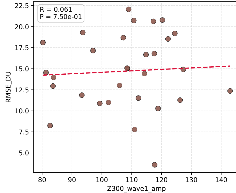
Z300_wave1_amp vs RMSE_DU
