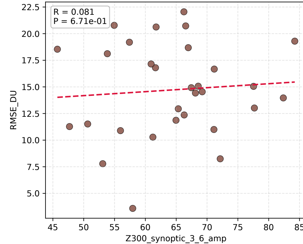
Z300_synoptic_3_6_amp vs RMSE_DU
