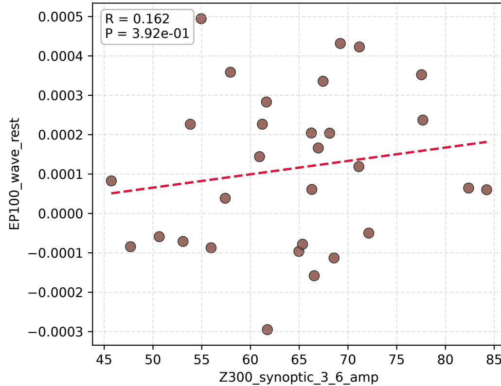
Z300_synoptic_3_6_amp vs EP100_wave_rest
