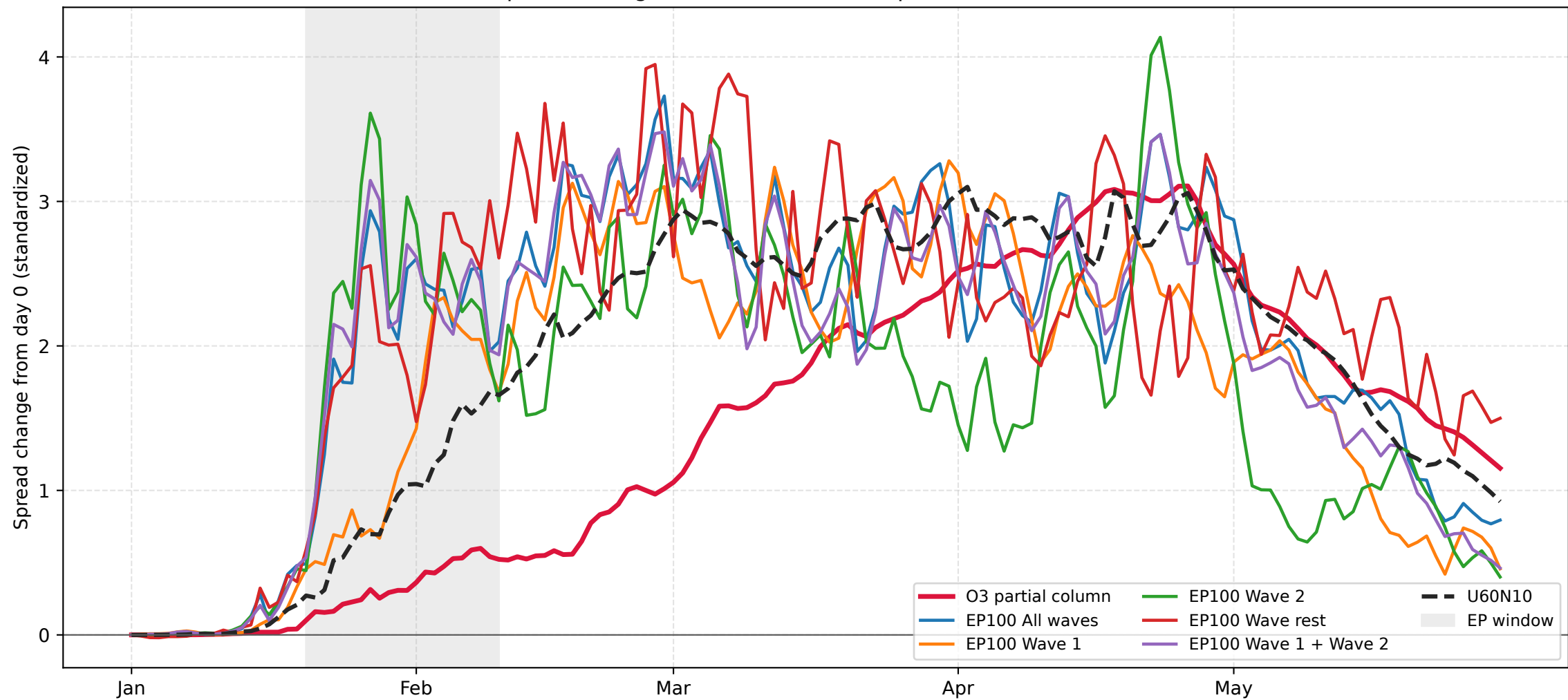
Spread timing: O3, EP100 wave components, and U60N10
