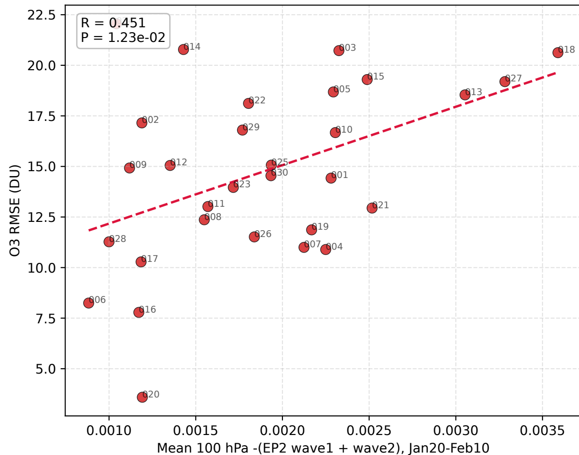
Wave1+Wave2 vs O3 RMSE
