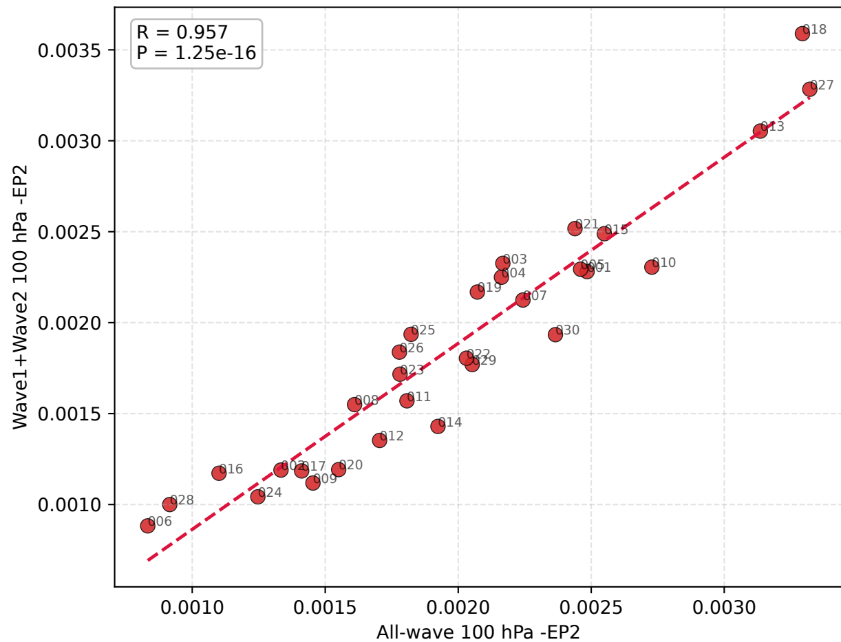
All-wave EP vs Wave1+Wave2 EP
