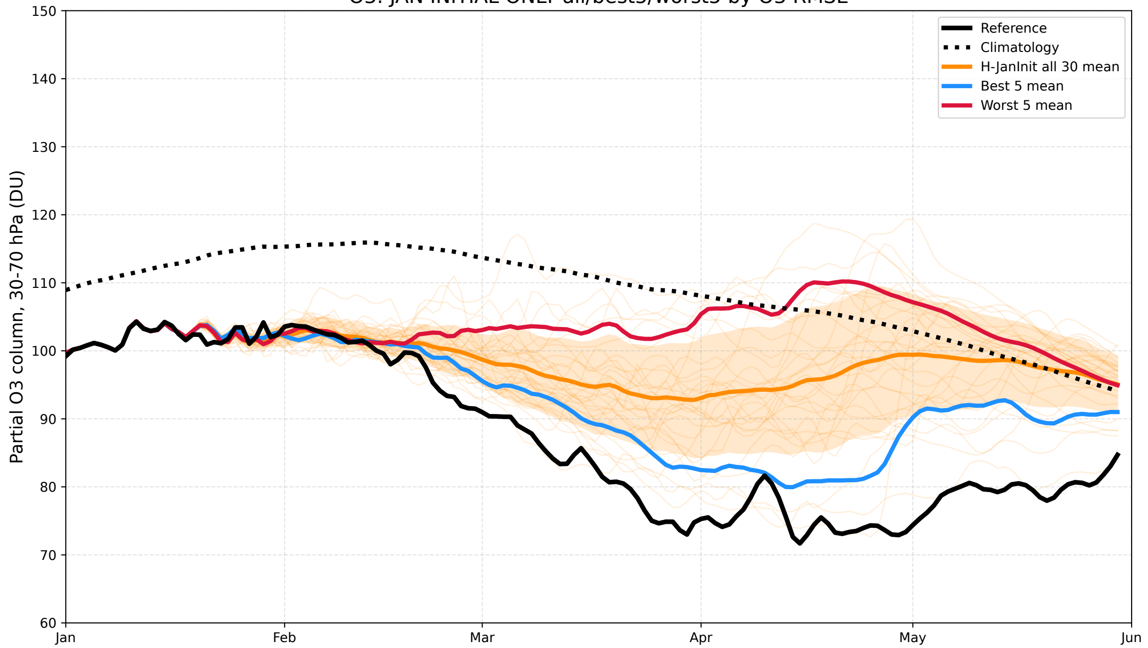
O3: JAN INITIAL ONLY all/best5/worst5 by O3 RMSE
