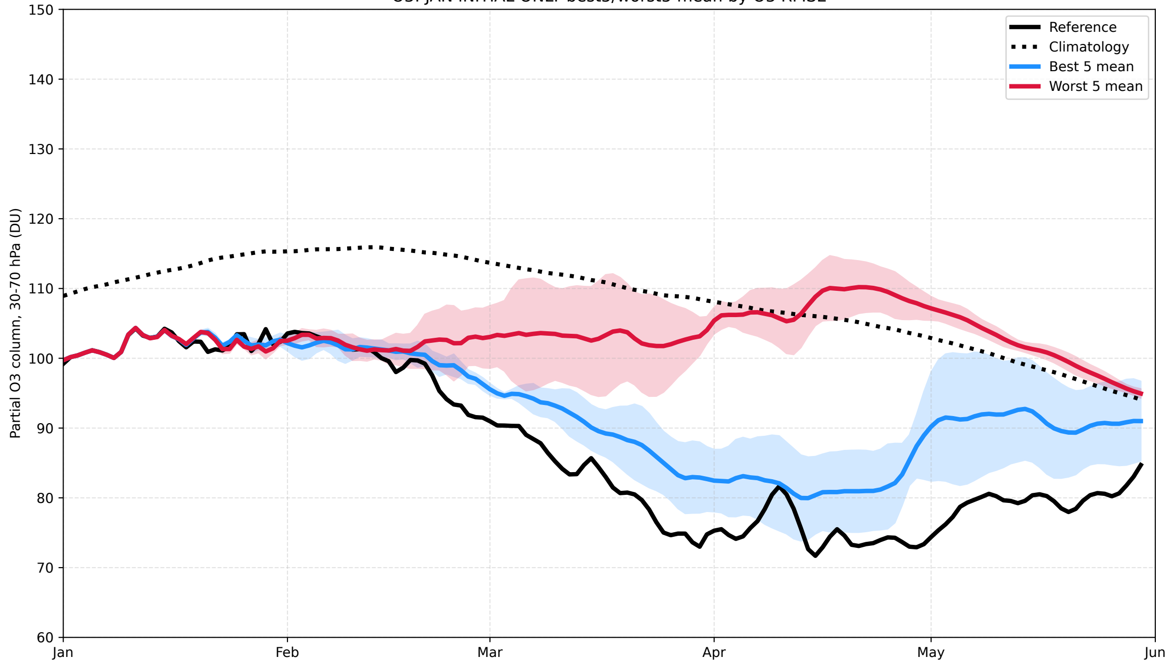
O3: JAN INITIAL ONLY best5/worst5 mean by O3 RMSE
