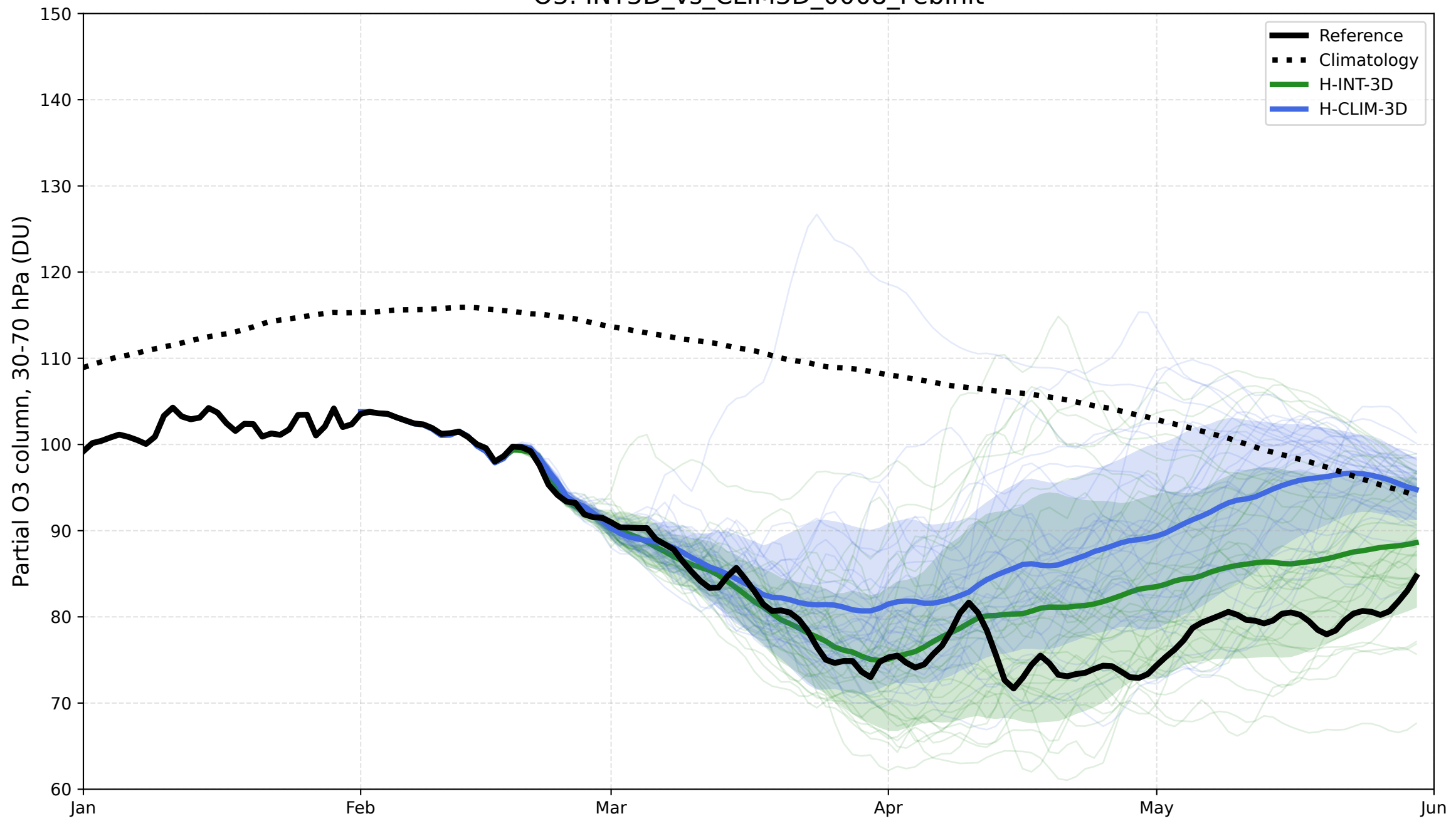
O3: INT3D_vs_CLIM3D_0008_FebInit
