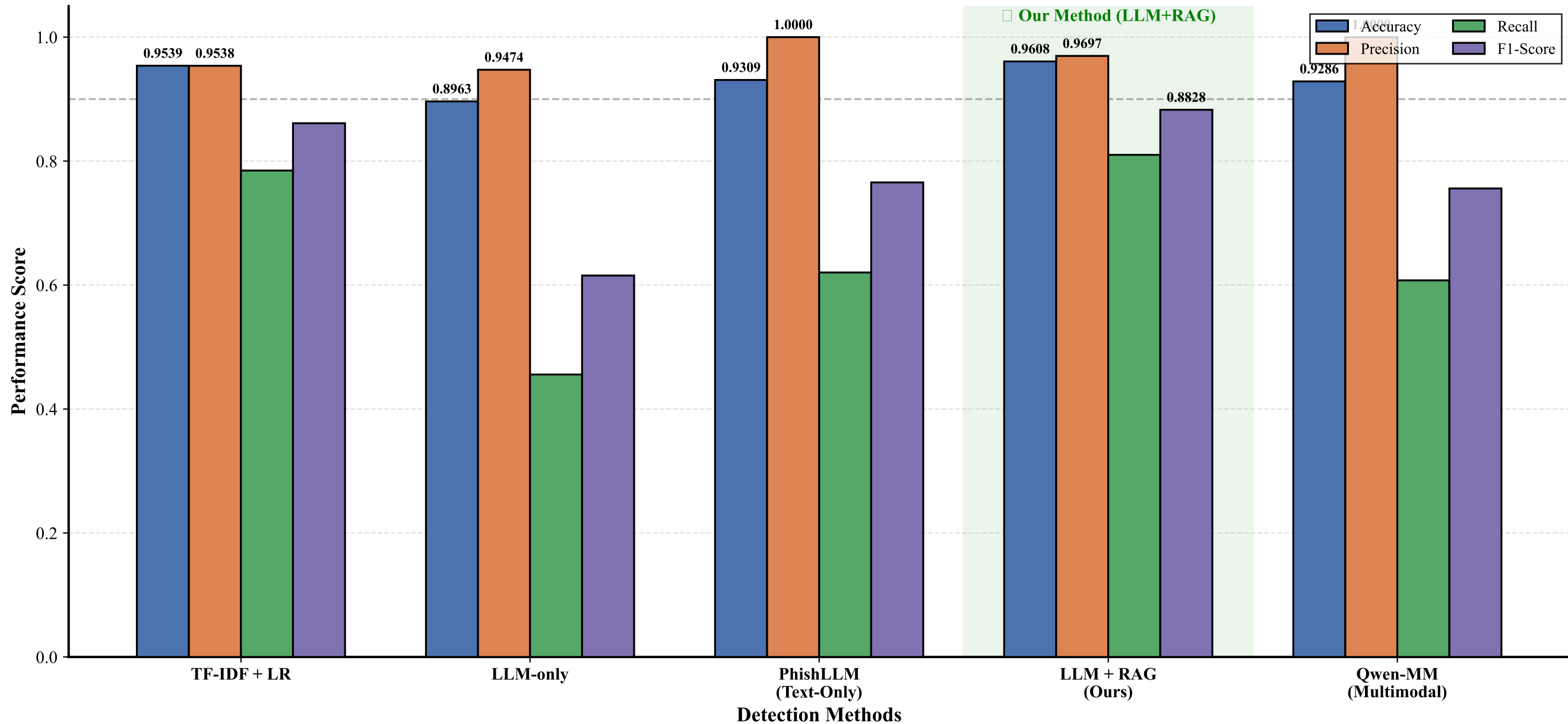
Figure 1: Performance Comparison of Phishing Detection Methods
